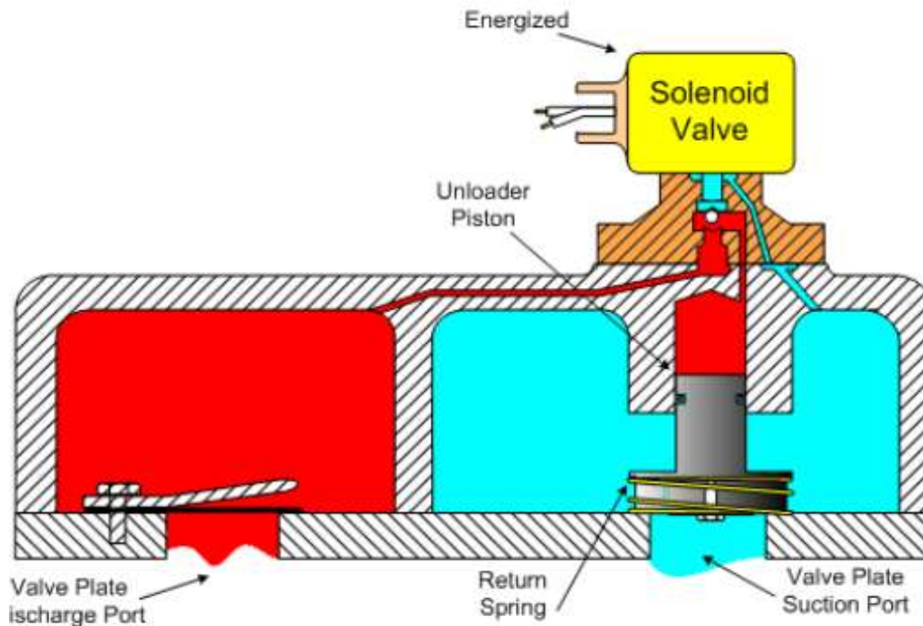
Unloader Piston in Unloaded Position
