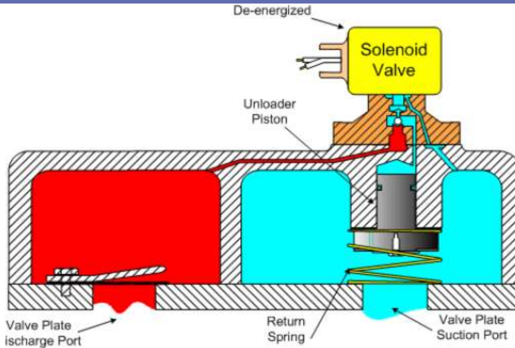
Unloader Piston in Loaded Position
